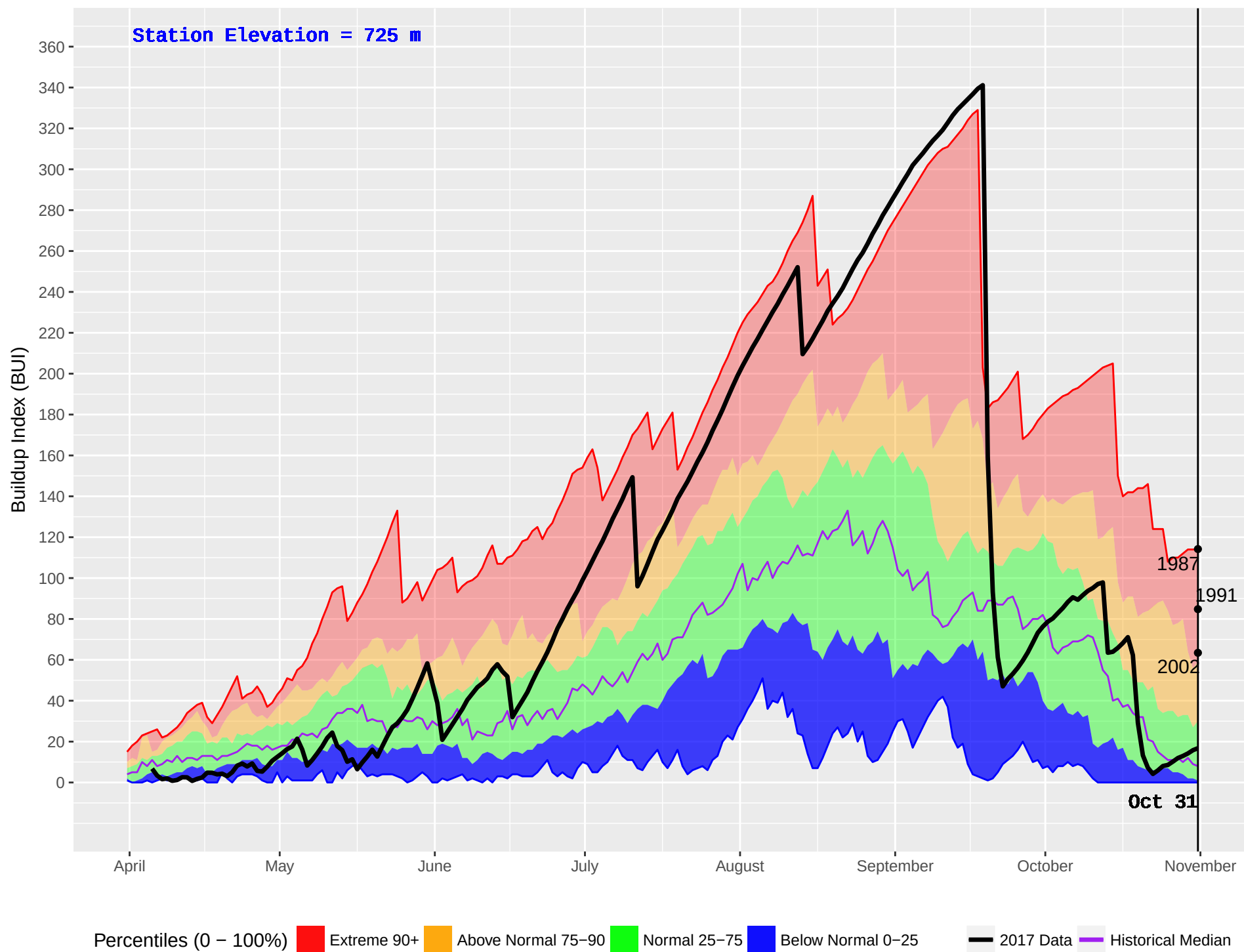
PENDOREILLE (402) : Historical (1986–2016) and Current (2017) Noon Buildup Index (BUI)
