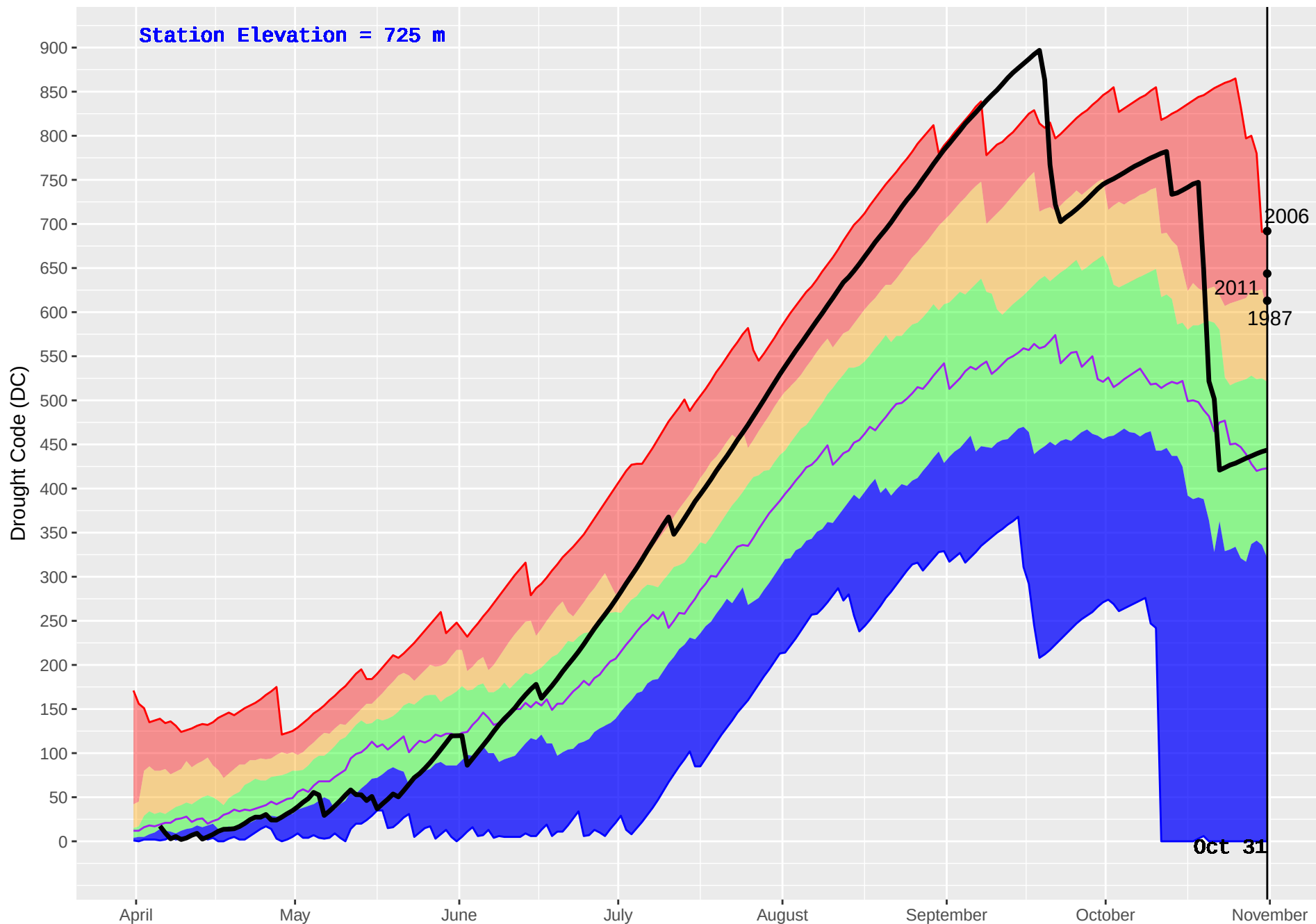
PENDOREILLE (402) : Historical (1986–2016) and Current (2017) Noon Drought Code (DC)
