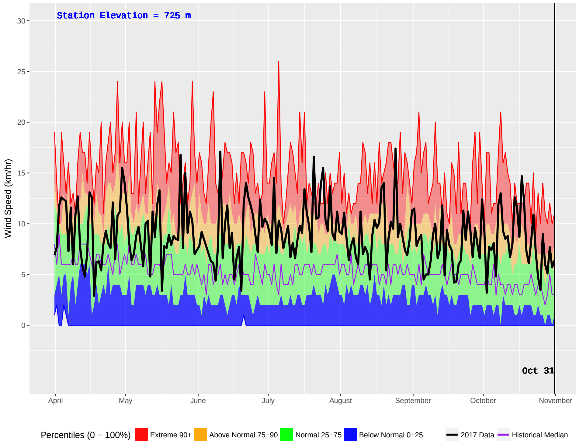
PENDOREILLE (402) : Historical (1986–2016) and Current (2017) Noon Wind Speed
